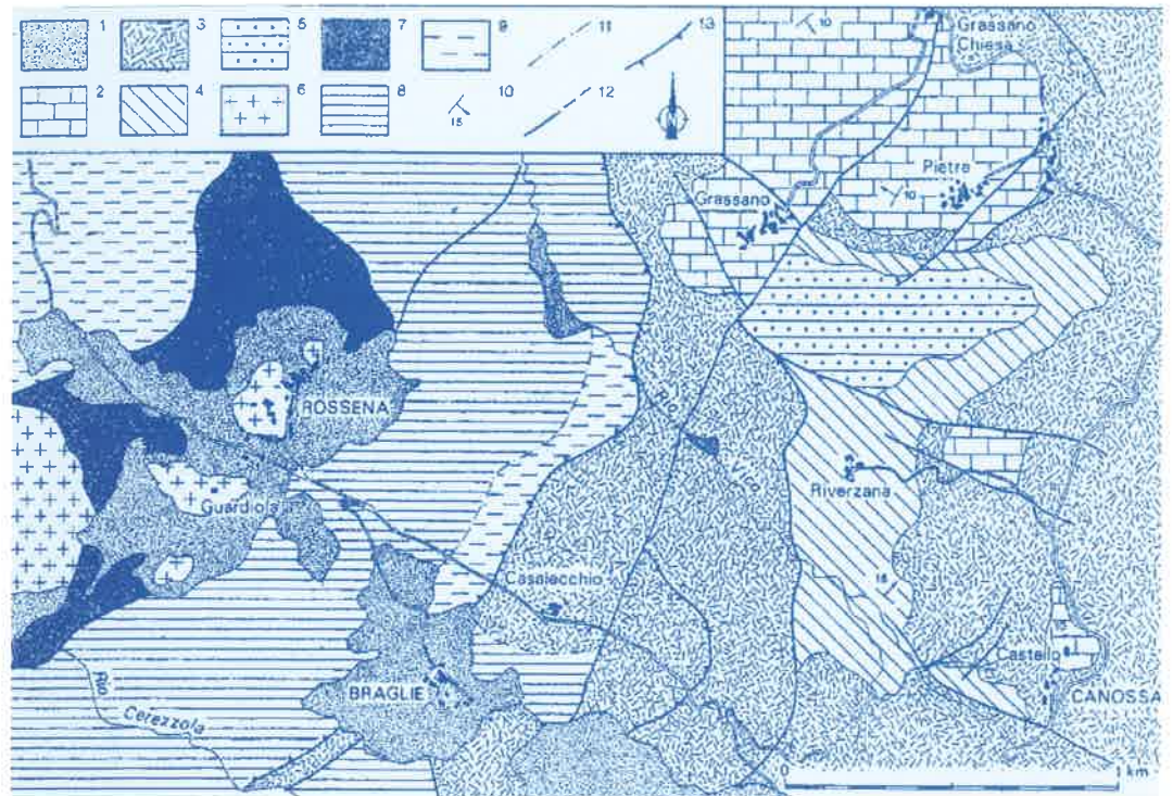
Figure 7 - Geologic sketch of the Rossena and Canossa surroundings. 1. Surficial Quaternary deposits; Epi-Ligurian Sequence; 2. Arenites from the Bismantova Group; 3. Canossa Olistostrome; 4. The Antognola Formation; 5. Ranzano Sandstone; 6. Rossena Ophiolites; 7. The Rossena Mélange; 8. Varicolored Shales; 9. Palombini Shales; 10. Dip of strata; 11. Uncertain boundary; 12. Faults; 13. Overthrust (after Bortolotti, 1994)
