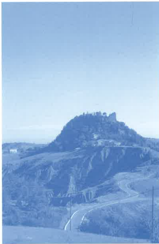
Figure 10 - The Canossa cliff (photo by P. Coratza)
