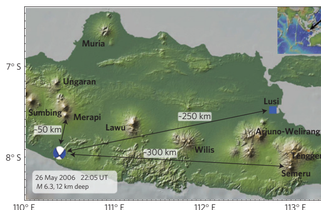
Figure 1 | Map of Java with relevant distances from the Yogyakarta earthquake. The blue square marks the position of Lusi and arrows show the distance between the epicentre of the Yogyakarta earthquake and the systems that responded to that event.
